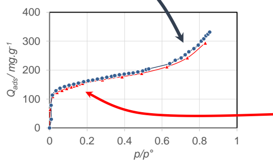
Cyclohexene@CoCo
