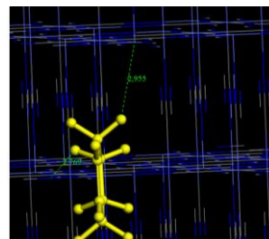
Cyclohexene@CoCo
