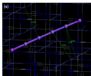
n -Hexane@CoCo
