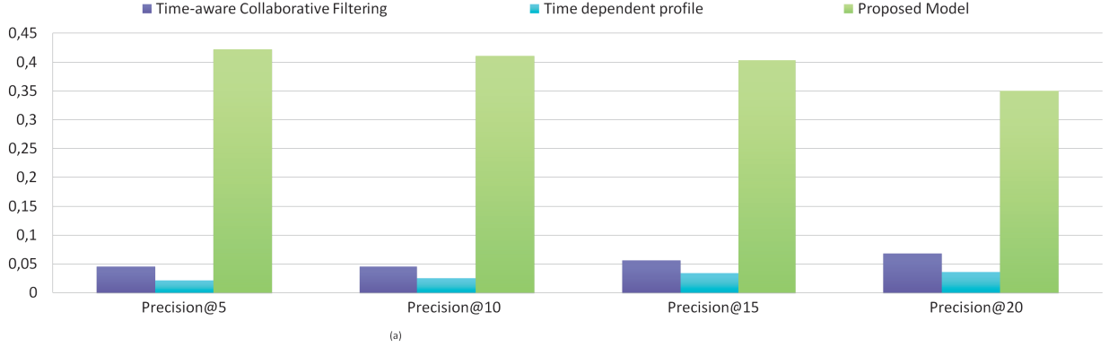
Fig. 1. Comparison with baseline models on Precision
