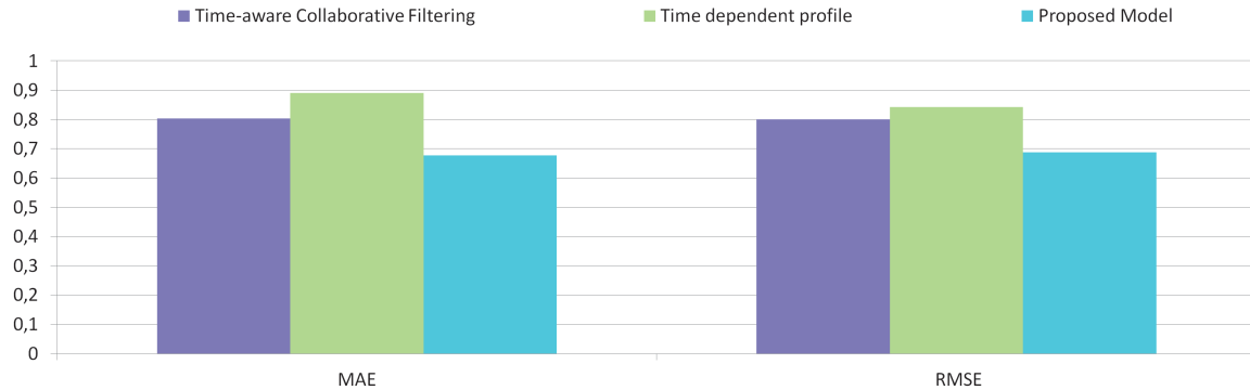
Fig. 2. Comparison with baseline models on MAE and RMSE
