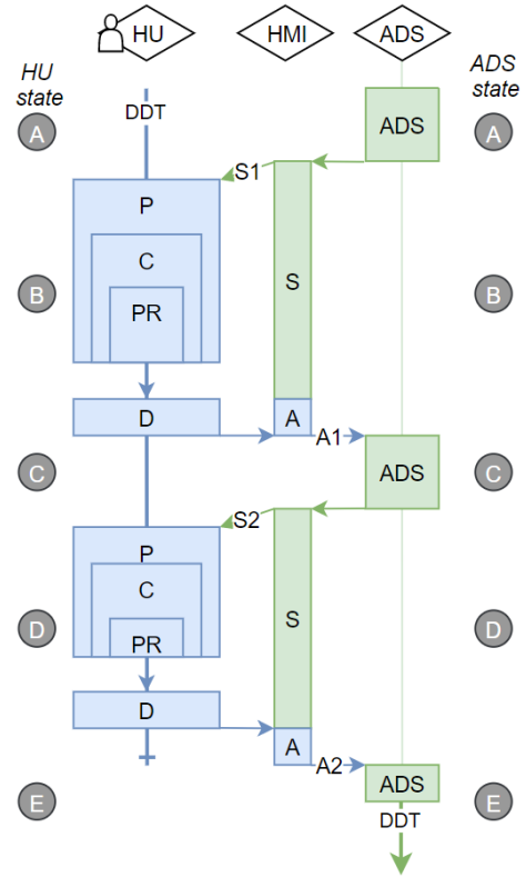
Fig. 10. The intended interaction sequence for T1 .
