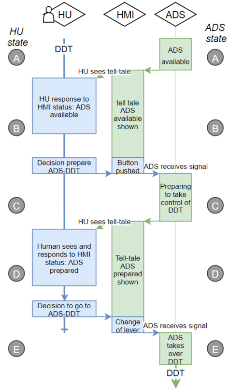
Fig. 11. Descriptive example of the intended interaction sequence for T1 .
