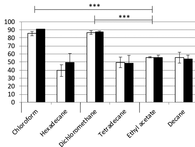
Fig. 5. Percentage affinity of Flavobacterium sp. II2003 cells to the six solvents used in the MATS method. Flavobacterium sp. II2003 cells were pretreated with SN_{IV2006} or Zobell broth (control). Three couples of solvents were used: chloroform (monopolar acidic)/hexadecane (apolar), dichloromethane (monopolar acidic)/tetradecane (apolar) and ethyl acetate (monopolar alkaline)/decane (apolar). Percentage affinities are mean values ( \pm SD) of five measures obtained from three independent treatments. Flavobacterium sp. II2003 cells, treated with SN_{IV2006} or Zobell broth, showed a significantly higher percentage affinity to the acidic solvents than to the alkaline solvent. These differences are indicated by *** ( P < 0.001 ).
