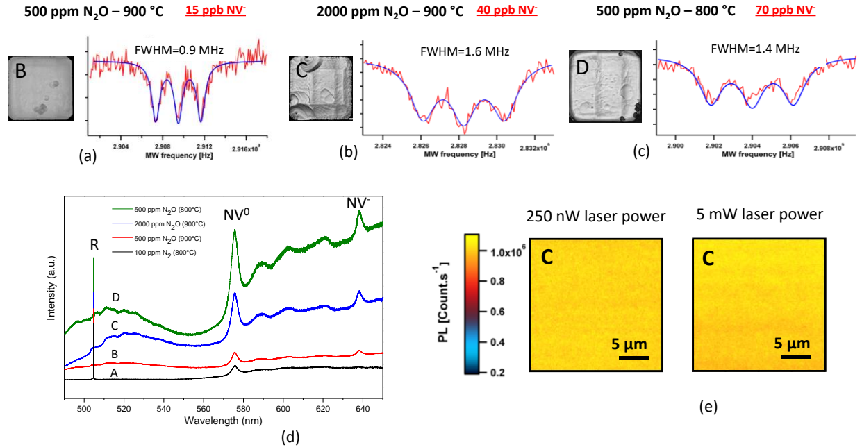
Fig. 3. (a)-(c) Laser microscope images of samples B, C and D grown with N 2 O addition and zoom into one of the hyperfine structures of the ODMR spectra showing the triplet and its linewidth. (d) Room temperature Raman/PL spectra (473 nm laser) for samples A, B C and D. Spectra were normalized to the Raman peak (labelled as R) and vertically shifted for clarity. The broader baseline around 520 nm originates from luminescence of the HPHT substrate underneath. (e) PL images obtained on sample C with a confocal scanning microscope (laser 532 nm) showing the perfect photostability of NV centres under higher laser powers.
