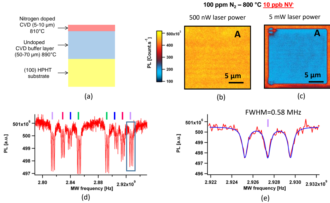
Fig .2. Optical properties of a thin film (sample A) grown with addition of 100 ppm of N 2 and a growth temperature of 800 °C. (a) Schematics showing the grown structure, (b) and (c) PL images obtained with a confocal scanning microscope (laser 532 nm) allowing estimating NV density and showing the poor photostability under high laser power. (d) ODMR spectra obtained under a magnetic field of 3 mT where 4 pairs of resonances are visible. (e) Zoom into one of the resonances highlighted by a square, where the characteristic hyperfine splitting is observed with a FWHM of 0.58 MHz.
