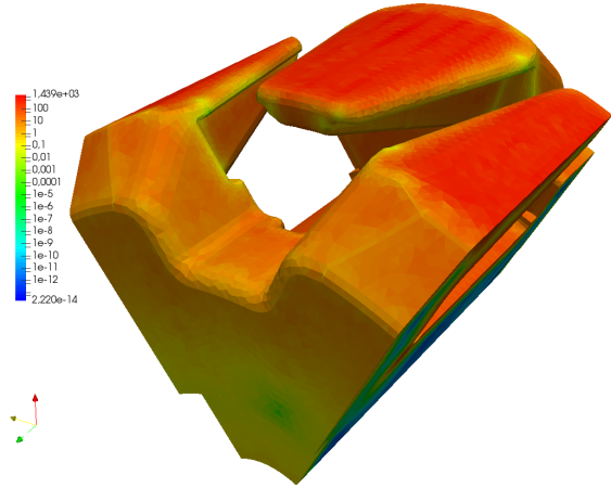
Fig. 4. Indicator of the areas where the variation of the magnetic vector potential is the greatest in the logarithm scale
