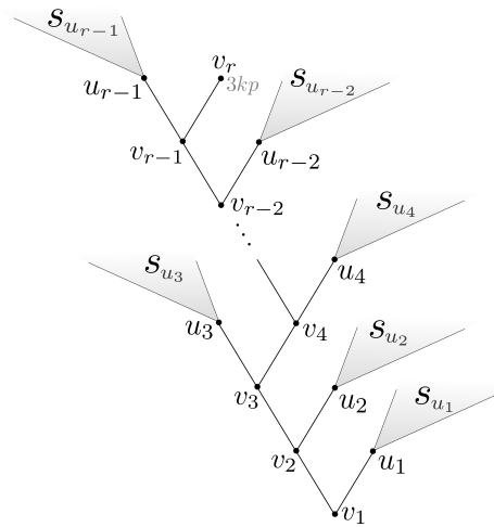
■ Figure 8 The path from the root v_1 to v_r , the leaf with position 3kp .
