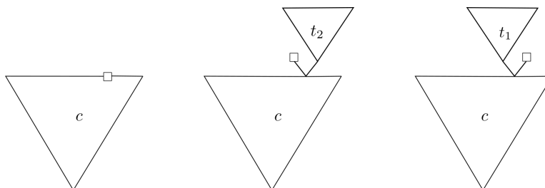
■ Figure 3 A context c , and the contexts c_{t_2}^1 and c_{t_1}^2 .
