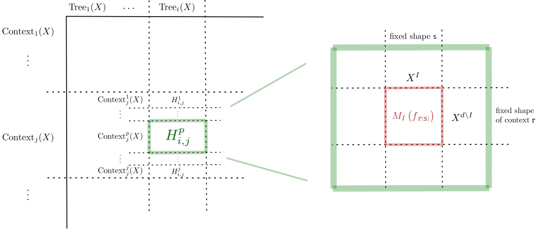
Figure 4 Decomposing H as blocks H_{i,j}^p , which further decompose into partial derivative matrices. Here, I denotes the interval [p, p + i - 1] .
