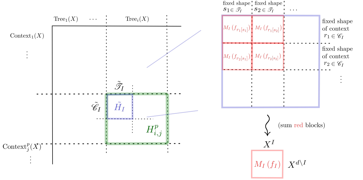
■ Figure 5 Decomposition of the Hankel matrix used in the proof of Lemma 28. Here, I = [p, p+i-1] .
