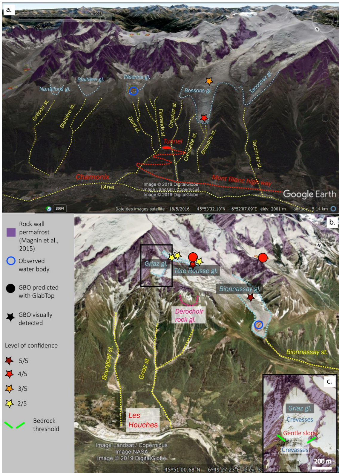
Figure 12. Example of potential hot spots in terms of risks based on already known active pro-glacial stream systems. a. General view of the Northwest face of the MBM. b. Focus on the Griaiz, Tête Rousse and Bionnassay glaciers and Les Houches village. c. Focus on the Griaiz glacier.
