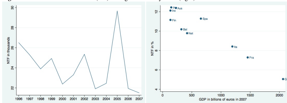
Fig. 1 New Trade Flows over time (left) and against country GDP (right)
