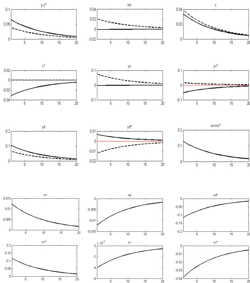
Fig. 2 IRF to a 1% domestic productivity shock (plain curves: the number of traded varieties evolves, dotted curves: the number of traded varieties is fixed)
