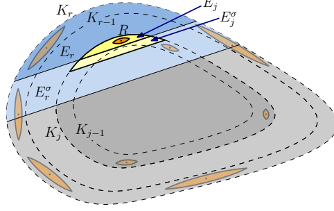
Figure 12: Proof of Lemma 5.13.
