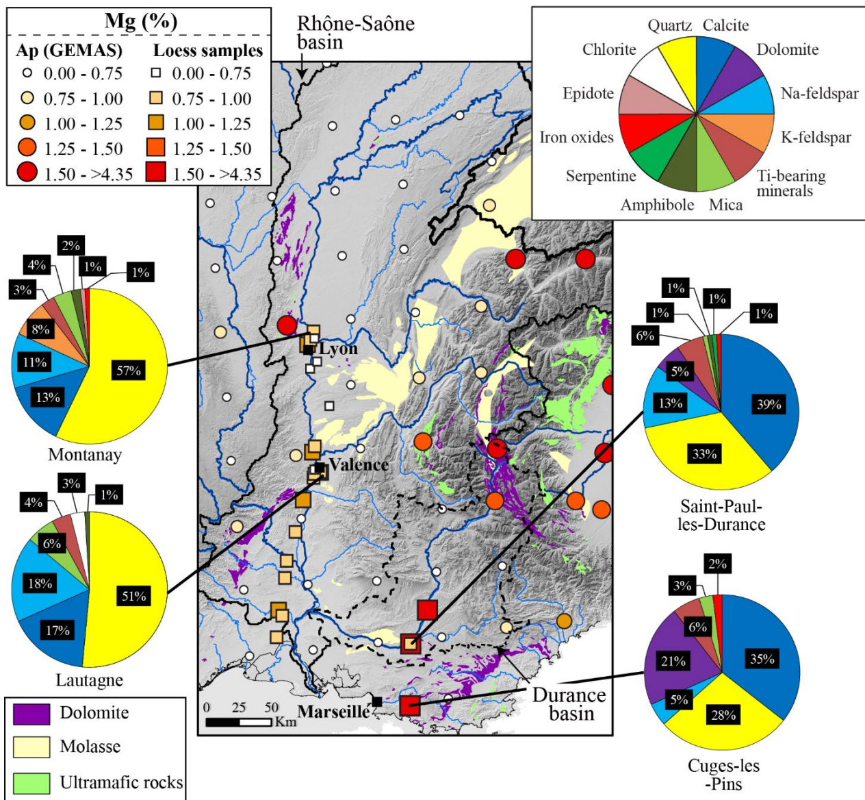
Fig. 3: Map of Mg content (expressed as a percentage) in loess samples and the ploughed soil layer, i.e., Ap horizon from GEMAS database (Reimann et al., 2014). Mineral assemblages and concentrations of the reference samples were analysed by Raman spectroscopy. The geological data were taken from the 1:1,000,000 harmonized geological map of Europe (INSPIRE) (Laxton et al. (2010) and the 1:5,000,000 International Geological Map of Europe (IGME) (Asch, 2003).
