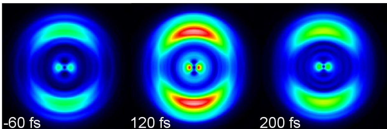
Figure 10. Photoelectron images at selected pump-probe delays, recorded at 324 nm, corresponding to excitation into the A^2A_1(3s) state. Figure reproduced from 189 . Copyright Journal of Physical Chemistry A.
