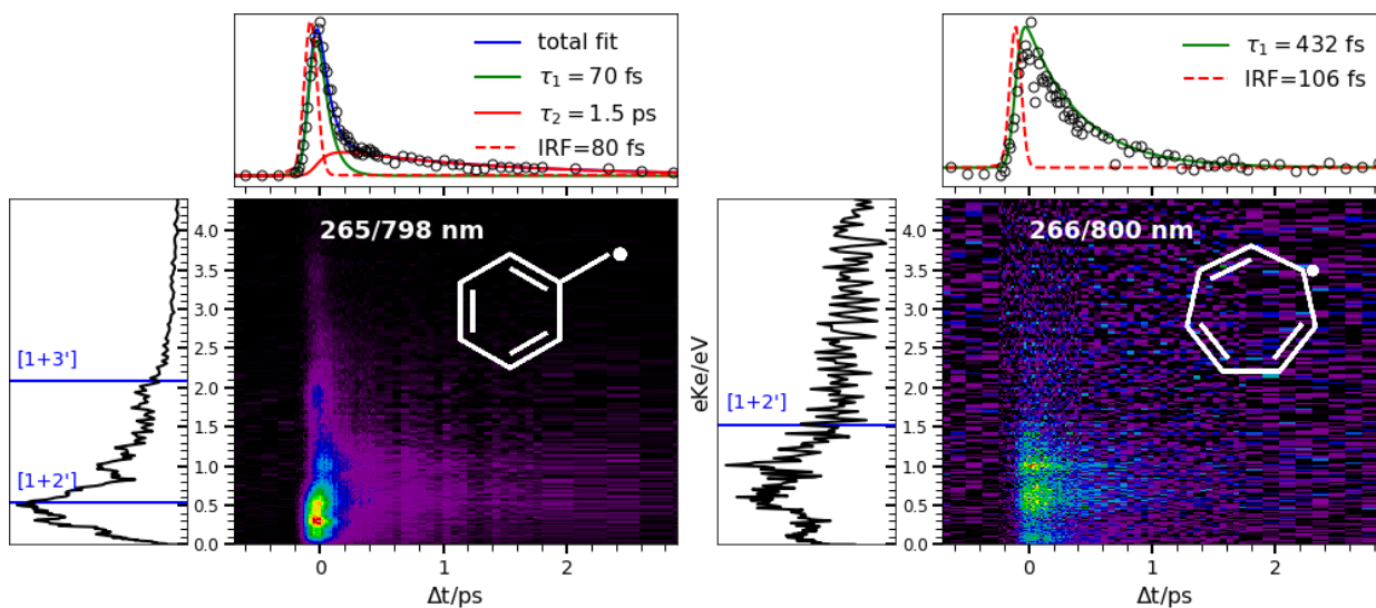
Figure 6. TRPES of the benzyl radical (left) and tropyl radical (right). The upper panels show the total photoelectron decay (experimental points: open black circles), fitted with either
