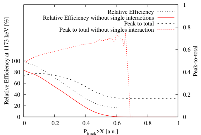
Figure 12: Efficiency relative to P_{\text{track}} = 0 at 1173 keV and peak to total as a function of P_{\text{track}} used by the OFT algorithm to accept or not a \gamma -ray track. This for when including or excluding single point interactions.
