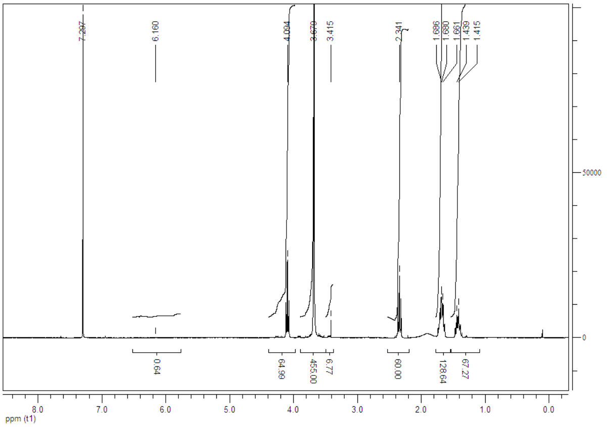
Fig. S2: 1 H NMR spectrum of crosslinked PEO-PCL micelle after freeze-drying and re-suspension in CDCl 3
