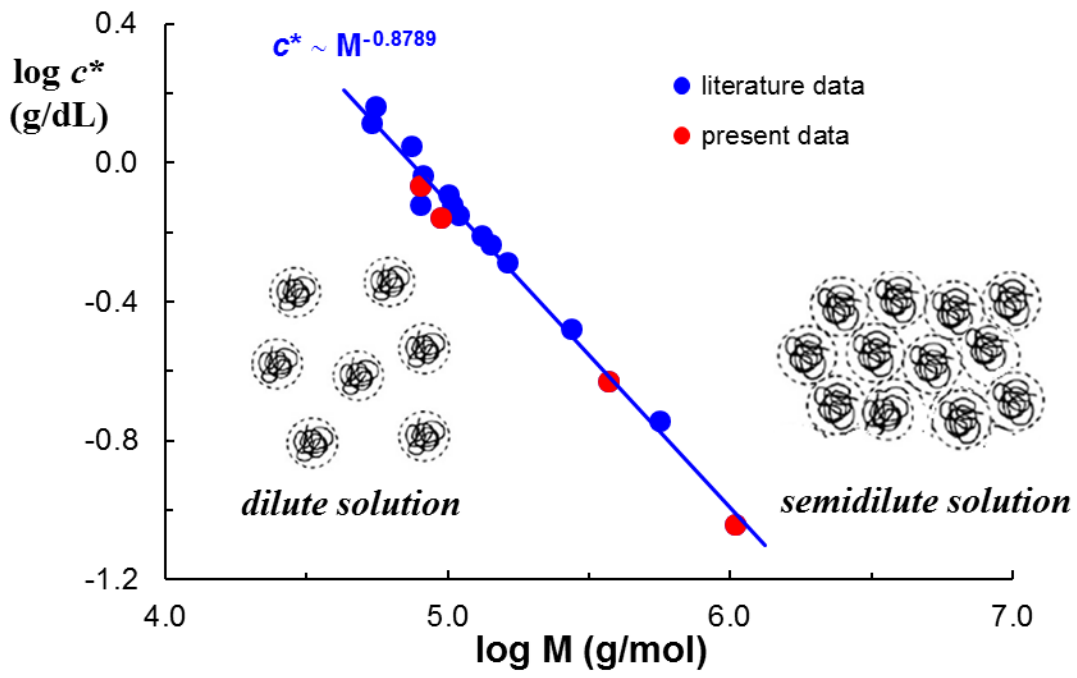
Figure 2. Delimitation of semi-dilute regimes for HPC aqueous solutions
