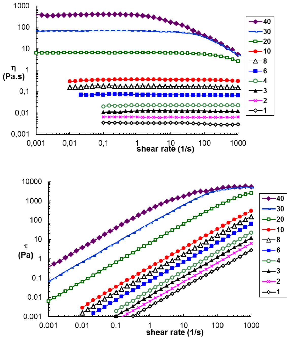
Figure 4: Flow curves for aqueous solutions of HPC with M = 8 \times 10^4 g/mol, different concentrations (g/dL) in water at 25°C
