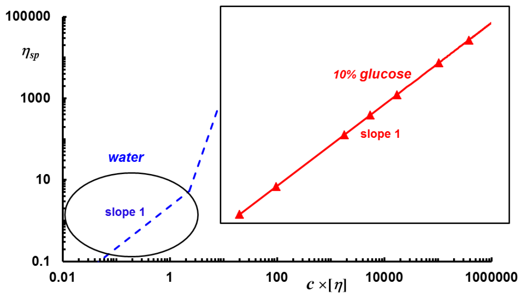
Figure 8: Regions where the linear dependence \eta_{sp} \sim c[\eta] was observed for HPC in different solvents at 25°C
