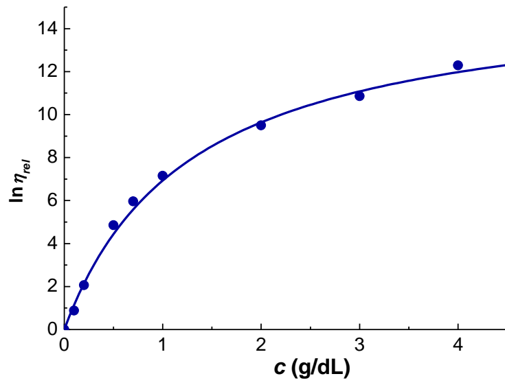
Figure 7: Plot of \ln \eta_{rel} as a function of c for HPC sample with M = 1.05 \times 10^6 g/mol in 10% glucose at 25°C. The curve is obtained by fitting the experimental data with equation (1)
