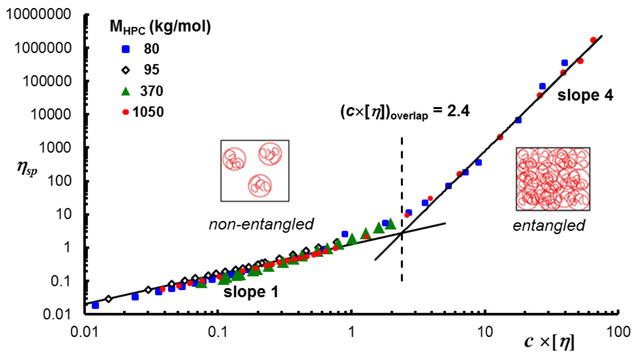
Figure 5: The specific viscosity as a function of c[\eta] for HPC of different molecular weights and concentrations in aqueous solution at 25°C
