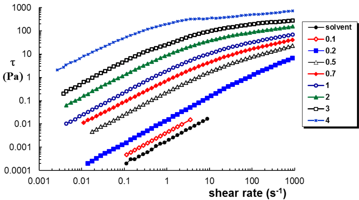
Figure 6: Flow curves for HPC sample with M = 1.15 \times 10^6 g/mol, different concentrations (g/dL) in 10% glucose aqueous solution at 25°C
