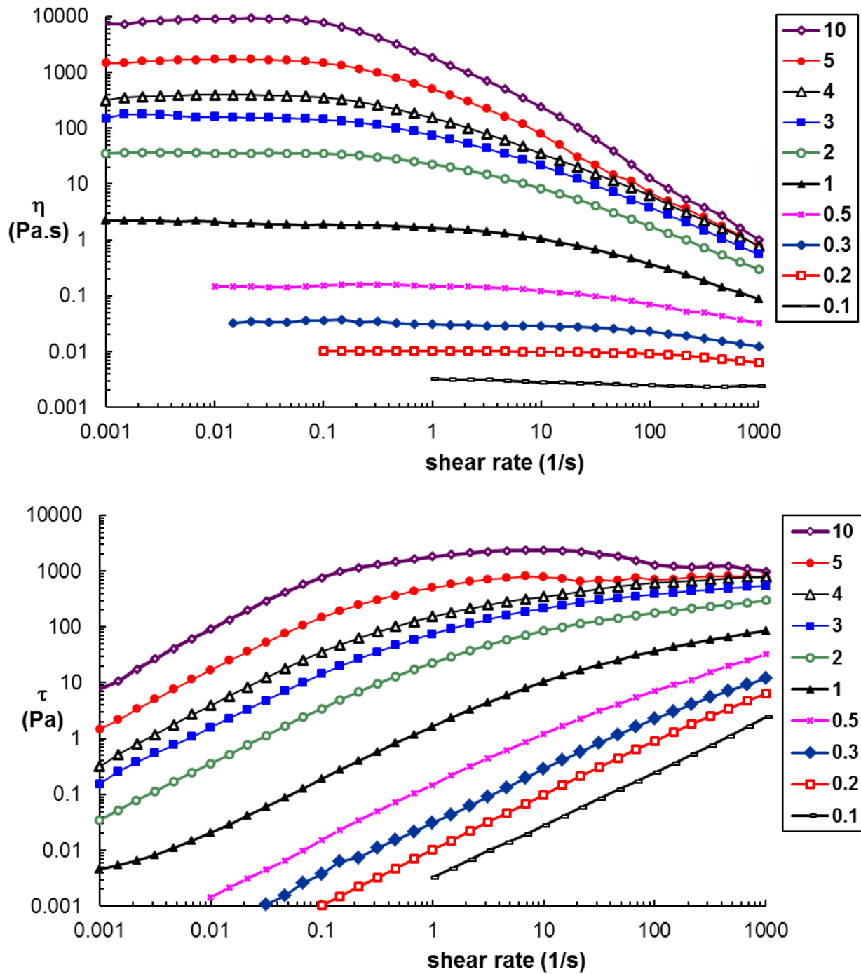
Figure 3: Flow curves for HPC sample with M = 1.15 \times 10^6 g/mol, different concentrations (g/dL) in water at 25°C
