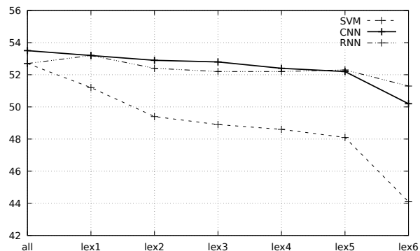
Fig. 1. Macro-F1 performance for SVM, CNN and RNN according to the lexicon size
