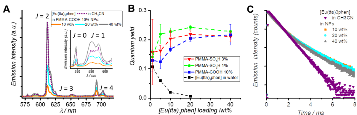
Figure 3. (A) Emission spectra ( \lambda_{exc} = 350 nm) recorded in aqueous solution for PMMA COOH 10% NPs loaded with different amounts of [Eu(tta) 3 phen], as well as of [Eu(tta) 3 phen] in CH 3 CN. Inset: Zoom on the ^5D_0 \rightarrow ^7F_{J=0,1} transitions. (B) Photoluminescence quantum yields of ECP-NPs vs [Eu(tta) 3 phen]-loading. Data points correspond to mean values from 3 independent measurements. Error bars correspond to SEM. ([Eu(tta) 3 phen] in water at 40 wt% led to formation of sedimenting aggregates.) (C) Time-resolved emission decay profiles (r.t., \lambda_{exc} = 350 nm) measured for solutions of [Eu(tta) 3 phen] in acetonitrile and of PMMA COOH 10% NPs loaded with different amounts of [Eu(tta) 3 phen]. Note: Log-scale for emission intensity.
