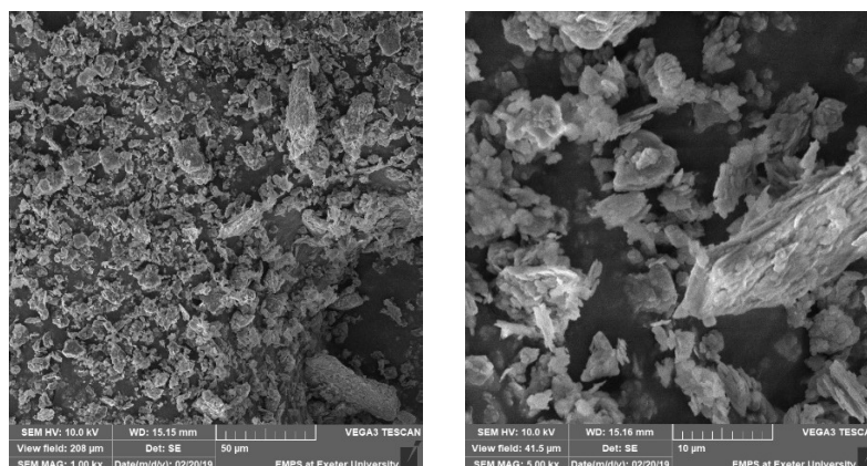
Figure 1 SEM images of pure kaolinite with 50 \mu m and 10 \mu m magnification factors
