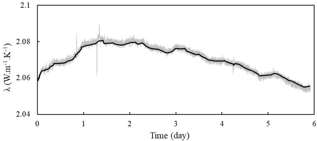
492 Figure 10 : Variation of the thermal conductivity \lambda ( \text{W. m}^{-1} \cdot \text{K}^{-1} ) during a centred hot plate 493 test on the compacted soil.
