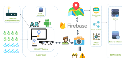
Figure 5. Global architecture
