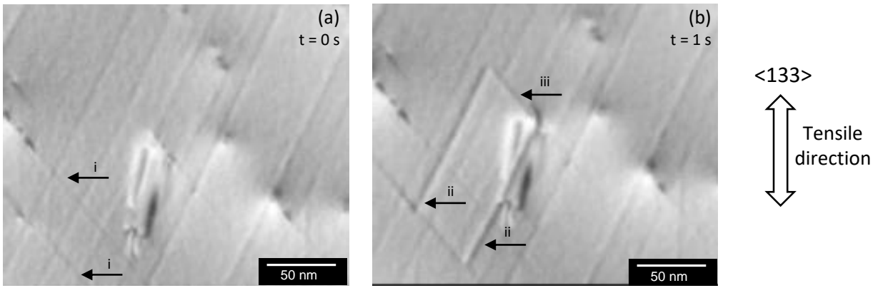
Figure 7: Video sequence of cross-slip at 200°C.
