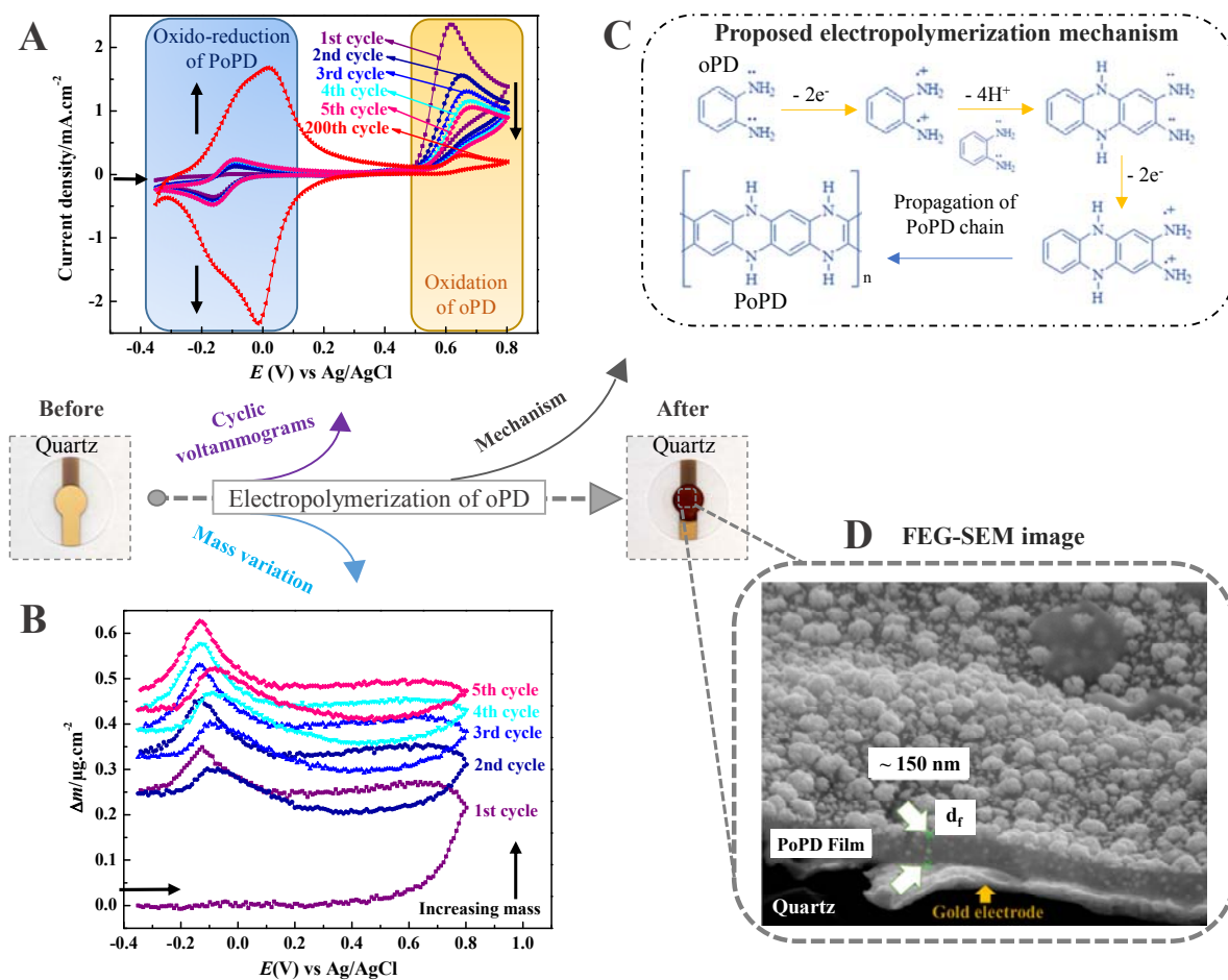
Fig. 1. PoPD thin film synthesis by electropolymerization on a gold electrode of a quartz resonator in an aqueous solution of \text{H}_2\text{SO}_4 (0.1 M) and oPD (5 mM). (a) CV Curves, (b) corresponding mass variations ( \Delta m ) obtained by EQCM at a scan rate of 50 \text{ mV}\cdot\text{s}^{-1} , (c) proposed electropolymerization mechanism and (d) FEG-SEM image of a PoPD thin film on the gold electrode of a quartz resonator after 200 CV cycles.
