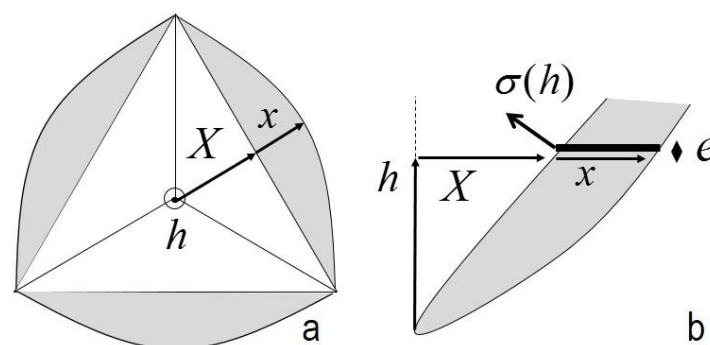
Figure 7. Scheme of a Berkovitch indent with the strained zone denoted in grey. (a) Top view, (b) cross-section view of a third of the indent. The parameters used in this modeling are as shown: indent shear X applied at height h , and the resulting shear displacement x of an NP infinitesimal thickness e . \sigma(h) was the resulting back stress produced at height h from the strain gradient.
