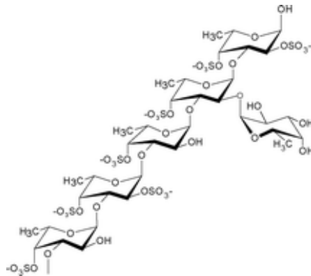
Figure 4: Schematic structure of fucoidan
