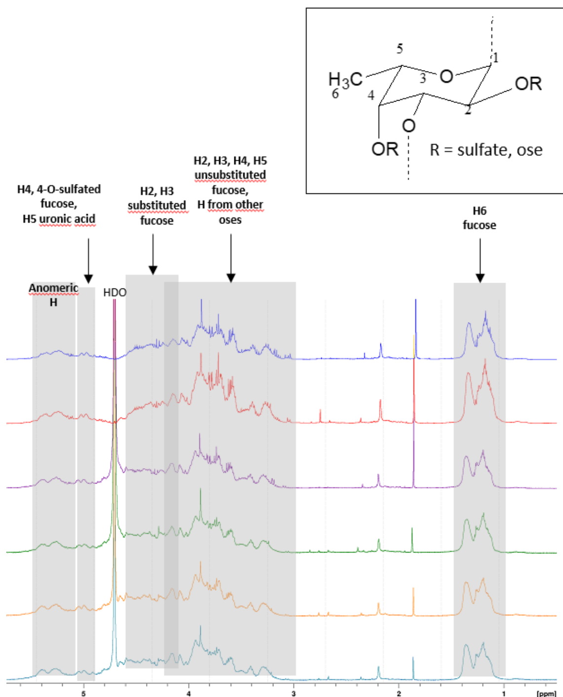
Figure 1: 1D- 1 H-NMR spectra of 6 API batches.
