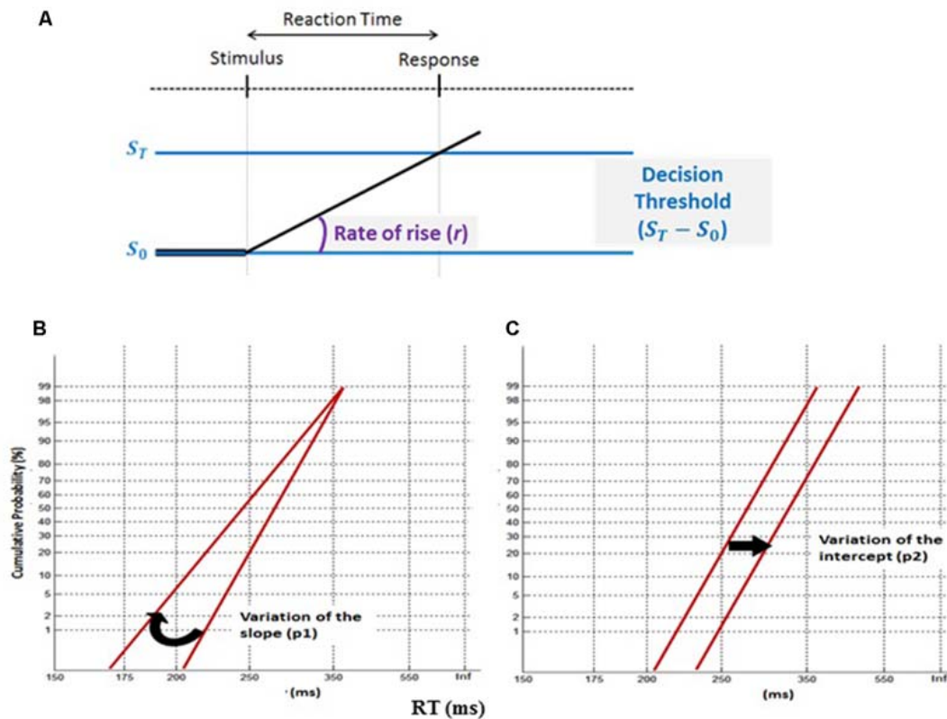
FIGURE 3 | The LATER model. (A) This decision-making model suggests that two mechanisms cause changes of mean reaction time (RT): a tonic modulation of the decision threshold ST - S_0 and a phasic change of the mean rate of rise ( r ). (B) A variation of the slope ( p1 ) between two conditions (swiveling in regard to the time axis) reveals a change in the model decision threshold, whereas, (C) a variation of the intercept ( p2 ) discloses a modulation in the rate of rise ( r ).
