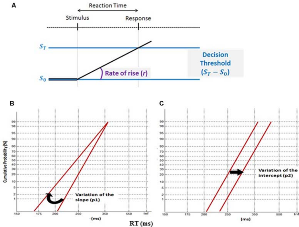
FIGURE 3 | The LATER model. (A) This decision-making model suggests that two mechanisms cause changes of mean reaction time (RT): a tonic modulation of the decision threshold S_T - S_0 and a phasic change of the mean rate of rise ( r ). (B) A variation of the slope ( p1 ) between two conditions (swiveling in regard to the time axis) reveals a change in the model decision threshold, whereas, (C) a variation of the intercept ( p2 ) discloses a modulation in the rate of rise ( r ).
