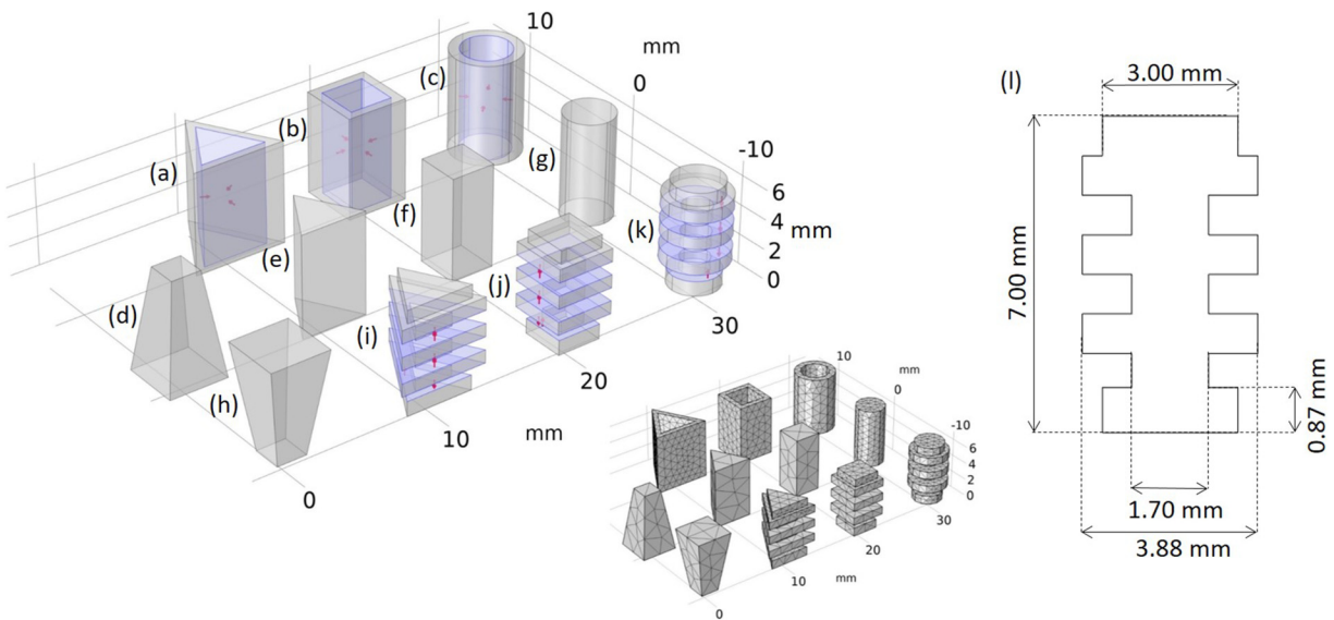
FIG. 2. Schematic of leg geometries modeled where the geometries are (a) triangular (hollow), (b) square (hollow), (c) circular (hollow), (d) trapezoidal (large base), (e) triangular (filled), (f) square (filled), (g) circular (filled), (h) trapezoidal (small base), (i) triangular (layered), (j) square (layered), and (k) circular (layered). The square (filled) geometry (f) approximates the conventional leg geometry. Arrows show the normal to the surface for the purposes of the radiation analysis. The inset shows the adaptive meshing used. (l) Schematic cross section of the square layered geometry.
