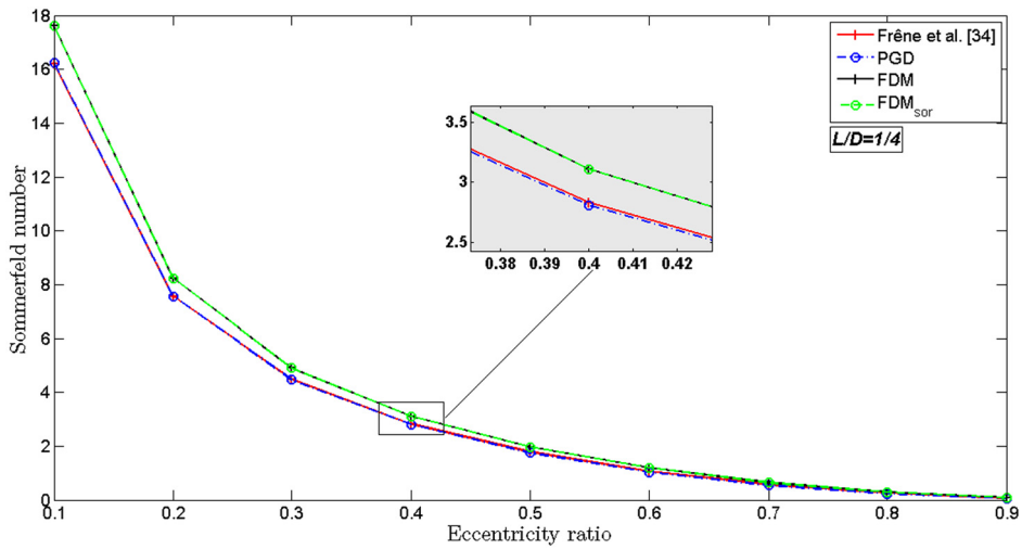
Fig. 22. Sommerfeld number with different values of the eccentricity ratio for FJB ( L/D = 1/4 ).
