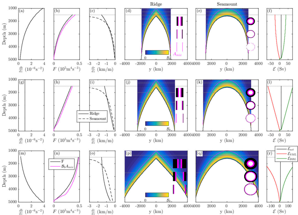
FIG. 5. As in Fig. 4, but for the (d),(j),(p) ridge and (e),(k),(q) seamount geometries. Note that above the crest of the topography (horizontal dotted lines) it is not possible to have net upwelling and thus F , dr/dz , and the diapycnal transports are not shown there.
