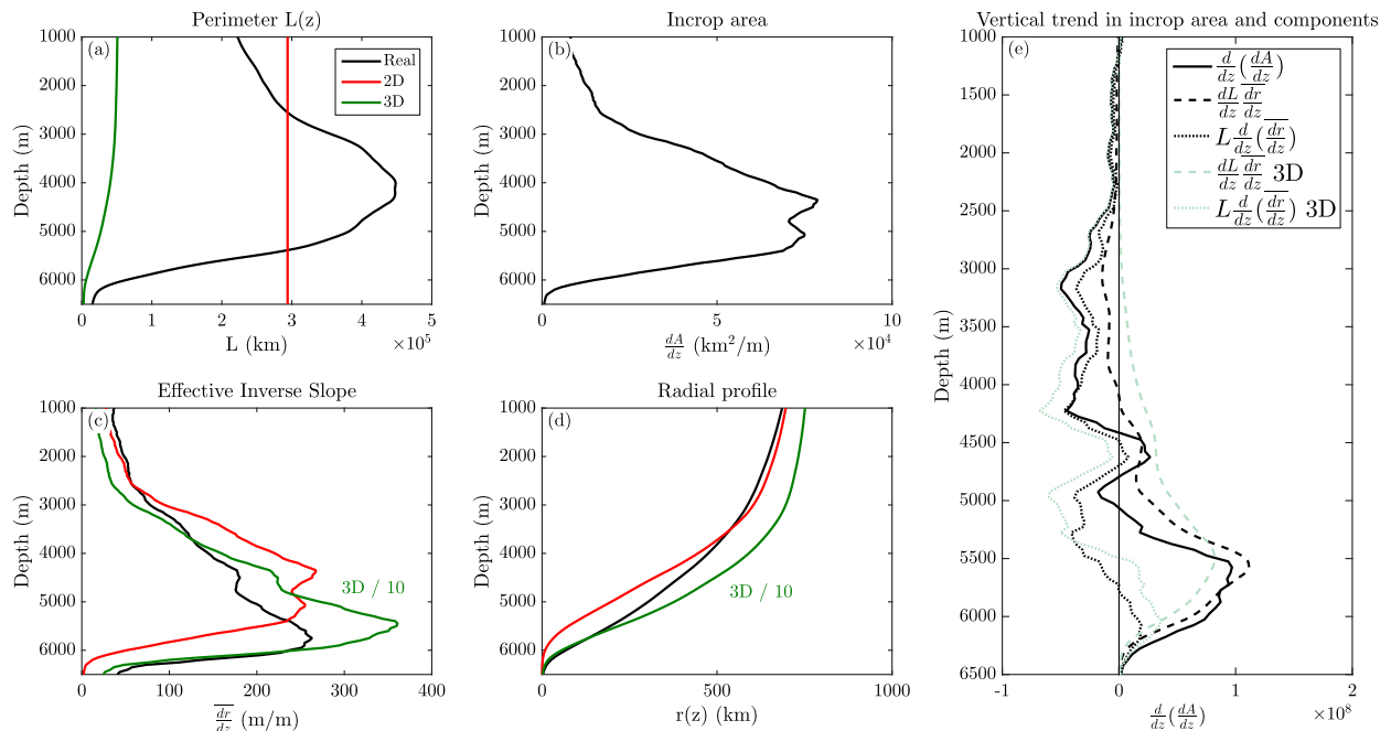
FIG. 11. Properties of the seafloor topography between 30°S and 48°N using 1/2° resolution topography. (a) Perimeter L(z) , (b) incrop area of depth layers, (c) the effective inverse slope \frac{dr}{dz} [Eq. (27)], (d) the radial profile obtained from \frac{dr}{dz} , and (e) the vertical trend in incrop area (solid black) and the contributions of variations in perimeter (dashed black) and inverse slope (dotted black) to that trend. In red is the 2D case where the perimeter is constant and equal to the average of the real perimeter. In green is the 3D axis-symmetric case characterized by L = 2\pi r [this case is also shown with faint lines in (e)]. Note the order of magnitude difference between the 3D case and the others in (c) and (d).
