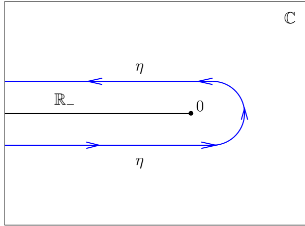
FIGURE 1. Hankel contour.
