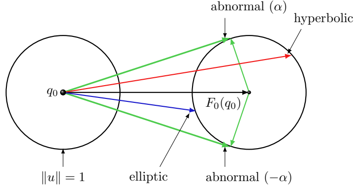
Figure 3: Strong current case: ball of directions.
