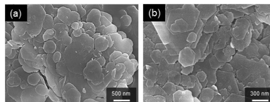
Figure 2. FE-SEM images of (a) 3S and (b) 3SF after Cl^- -exchange treatment.
