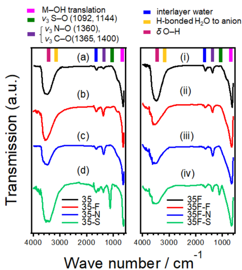
Figure 7. FT-IR spectra of LDHs: (a) 35, (b) 35-F, (c) 35-N, (d) 35-S, (i) 35F, (ii) 35F-F, (iii) 35F-N, and (iv) 35F-S.
