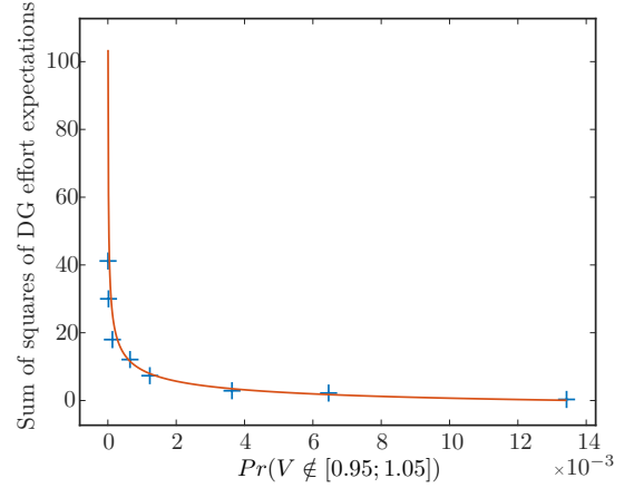
Figure 10. Pareto barrier
