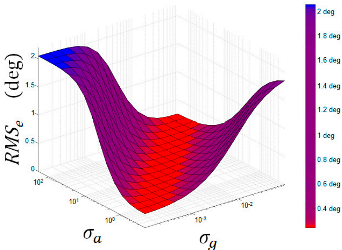
Figure A2. RMS_e between the orientation estimated with the optoelectronic system and the Kalman filter depending on the values of Kalman parameters \sigma_g and \sigma_a for the slow intensity movement.
