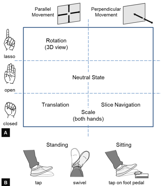
Fig. 4. Interaction Space: (a) User actions mapped according to hand gesture and movement's direction relative to the screen of the proposed touchless interaction system; (b) Feet gestures considered while the user is standing (tap and swivel) and sitting (tap on the foot pedal).
