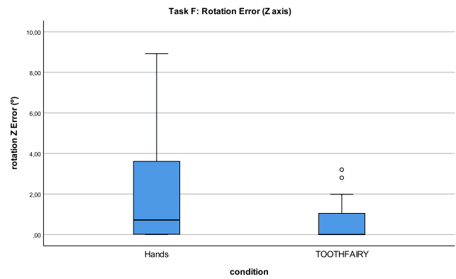
Fig. 12. Rotation-Z Error for Baseline (hands-only) and TOOTHFAIRY conditions in Task F.
