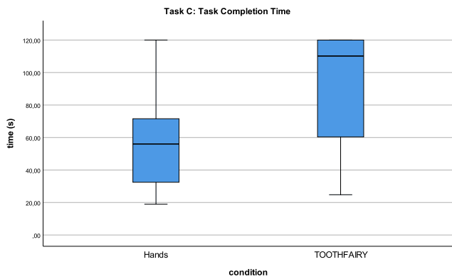
Fig. 9. Task completion time for Baseline (hands-only) and TOOTHFAIRY conditions in Task C.
