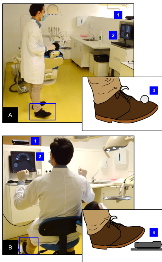
Fig. 1. The setup of the TOOTHFAIRY prototype includes (1) a depth camera to capture gesture interaction and (2) a display monitor for the graphical user interface. Regarding feet input, the prototype considers (A) a standing condition, which requires the use of (3) an optical marker, and (B) a sitting condition, which uses a foot pedal instead.
