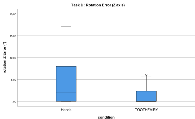
Fig. 11. Rotation-Z Error for Baseline (hands-only) and TOOTHFAIRY conditions in Task D.
