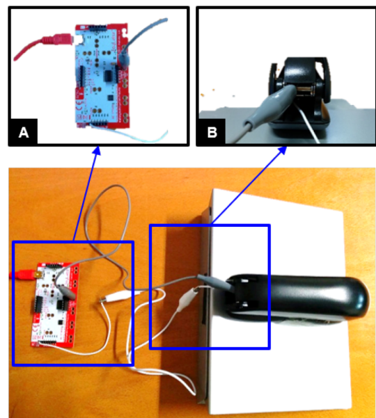
Fig. 5. TOOTHFAIRY setup using Makey Makey: (A) the Makey Makey board is connected via a USB cable (red) to the laptop PC; the white cable is connected to the board's keyboard input, while the grey cable is connected to the board's ground; (B) each cable is attached to a metallic part of the stapler, one to the upper (grey) and one the lower part (white), to allow the stapler to work as a switch. (For interpretation of the references to colour in this figure legend, the reader is referred to the web version of this article.)
