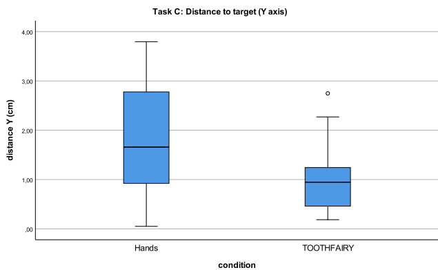
Fig. 10. Distance-Y to the target for Baseline (hands-only) and TOOTHFAIRY conditions in Task C.
