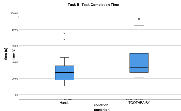
Fig. 8. Task completion time for Baseline (hands-only) and TOOTHFAIRY conditions in Task B.
