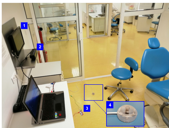
Fig. 6. TOOTHFAIRY 2.0 setup in the dental treatment room: (1) Monitor display; (2) Depth camera; (3) Makey Makey board; (4) Foot pedal.
