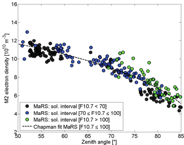
Fig. 14 Observed (circles) and modeled (dashed line) peak densities for the main ionospheric layer, as a function of the solar zenith angle. The color of the circles indicates the interval of solar activity. The density varies as \cos 0.44 (SZA), while a pure photochemical layer would follow a \cos 0.5 expression. The figures are adapted from Peter et al. (2014)
