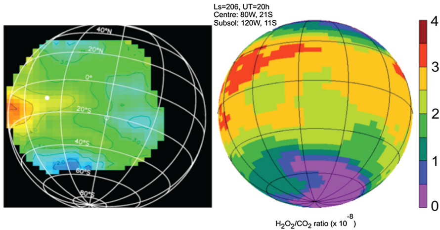
Fig. 11 Left map of the \text{H}_2\text{O}_2/\text{CO}_2 mixing ratio, derived from the line depth ratio of weak \text{H}_2\text{O}_2 and \text{CO}_2 transitions near 8\ \mu\text{m} , obtained from data recorded by the TEXES imaging spectrometer at the Infrared Telescope facility (IRTF) in June 2003 (MY 26, L_s = 206^\circ ). The subsolar point is indicated with a white dot . The \text{H}_2\text{O}_2 mixing ratio is indicated by multiples of 10^{-8} ; contours are separated by 0.5 \times 10^{-8} . Right map of the \text{H}_2\text{O}_2 mixing ratio, in the same unit, as modeled by the GCM developed at the Laboratoire de Météorologie Dynamique, under the conditions of the TEXES observations. The figures are taken from Encrenaz et al. (2004)
