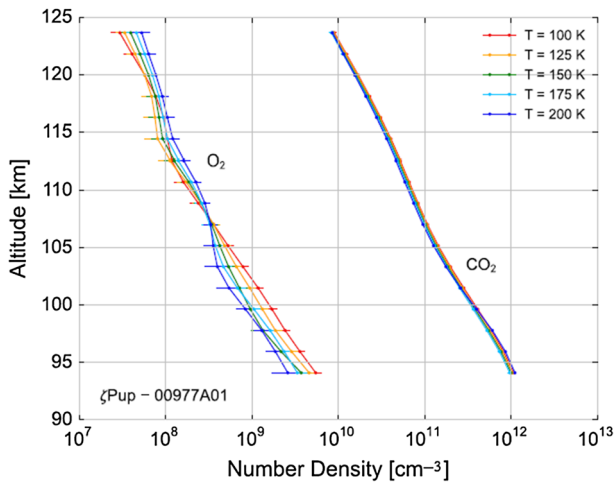
Fig. 13 CO 2 and O 2 abundances retrieved from stellar occultations. Over the range of 90–130 km, the altitude-averaged mixing ratio of O 2 relative to the major constituent CO 2 varies in space and time in the range of 3.1 \times 10^{-3} – 5.8 \times 10^{-3} , with a mean value of 4.0 \times 10^{-3} . This mean value exceeds by a factor of 3–4 those reported earlier for the lower atmosphere. However, some of the O 2 abundance and mixing ratio profiles determined here are similar to those measured by Viking in 1976 in the upper atmosphere. The figures are taken from Sandel et al. (2015)
