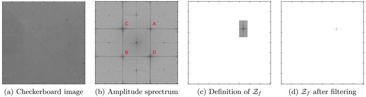
Figure 2: Selection of a region \mathcal{Z}_f around the fundamental peak of a checkerboard image in the Fourier domain. (a): Typical checkerboard image. (b): Amplitude spectrum of the checkerboard image. (c) Selection of \mathcal{Z}_f . (d): \mathcal{Z}_f after filtering by thresholding the coefficients ( k = 80\% ).
