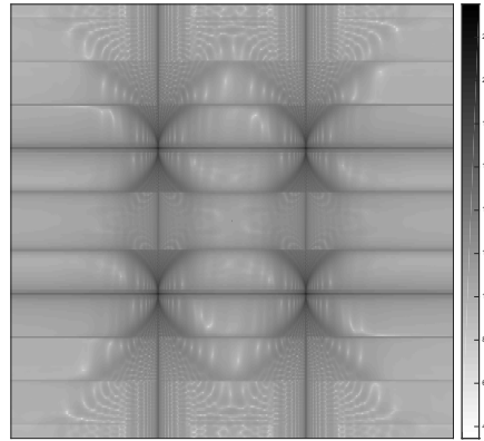
(b) spectrum of noiseless deformed checkerboard
