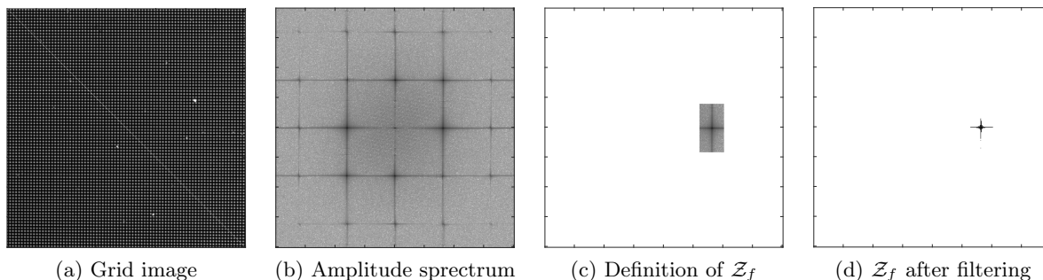
Figure 1: Selection of a region \mathcal{Z}_f around the fundamental peak of a grid image in the Fourier domain. (a): Typical grid image. (b): Amplitude spectrum of the grid image. (c) Selection of \mathcal{Z}_f . (d): \mathcal{Z}_f after filtering by thresholding the coefficients ( k = 80\% ).
