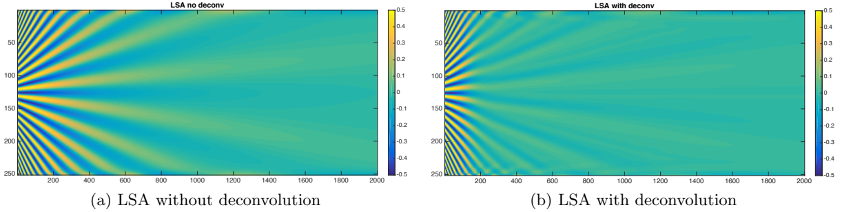
Figure 14: Maps of residual \delta u_y^{\text{LSA}} . The window w used with LSA is the same as the zone \mathcal{Z}_r used with WGPA in Figure 12. This is a Gaussian envelope of standard deviation \sigma = 6 pixels.
