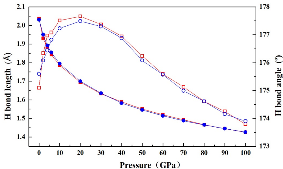
Figure 8. Lengths (solid symbols) and angles (open symbols) of the two H-bonds (red squares: \text{N3-H1}\cdots\text{N2} , blue circles: \text{N3-H2}\cdots\text{N2} ) in the \text{AA-P2}/c structure as a function of pressure, as obtained by present DFT calculations.
