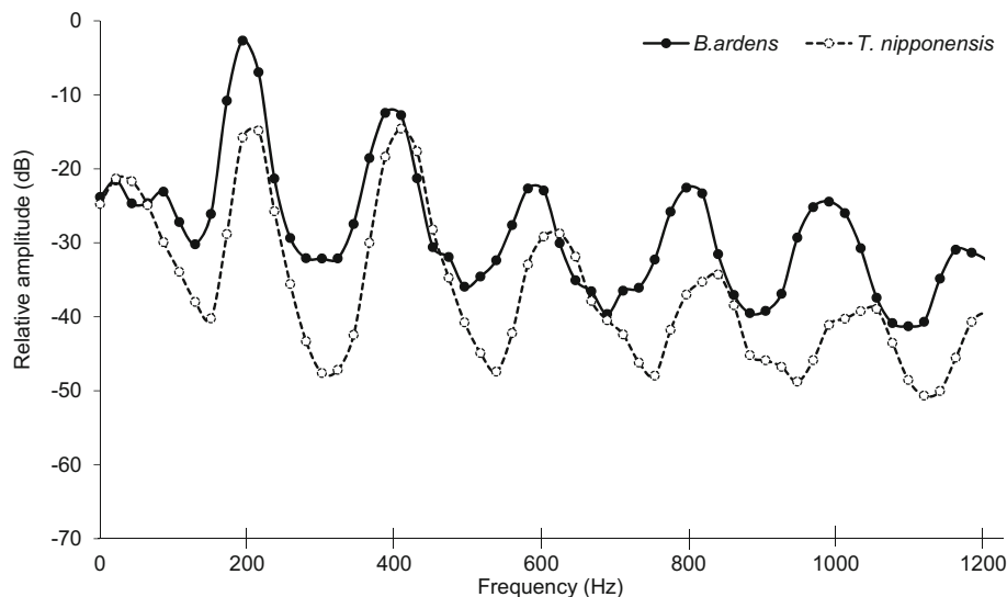
Figure 2 Example of a frequency spectrum of flight sounds of Bombus ardens and Tetralonia nipponensis .
