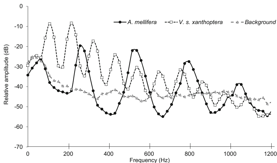
Figure 1 Example of a frequency spectrum of flight sounds of Apis mellifera , Vespa simillima xanthoptera , and background sounds.
