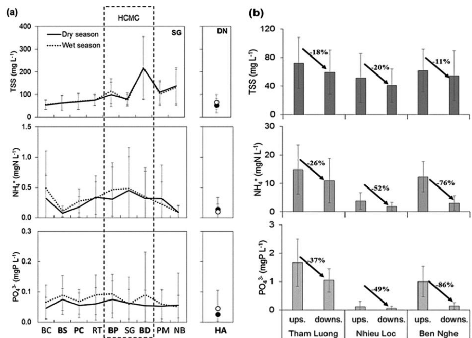
FIGURE 2 Mean total suspended sediment (TSS), NH 4 + , and PO 4 3- concentrations over the 2012–2016 period: (a) along the Saigon River (SG) and the Dongnai River (DN) during the wet and dry seasons and (b) in urban canals of Ho Chi Minh City (HCMC); BC, BS, PC, RT, BP, SG, BD, PM, NB, and HA are 10 sampling sites within the Saigon-Dongnai River basin (Ben Cui, Ben Suc, Phu Cuong, Rach Tra, Saigon, Bach Dang, Phu My, Nha Be, and Hoa An, respectively). In Figure 2a, bold legends represent sampling sites chosen for the budget calculation
