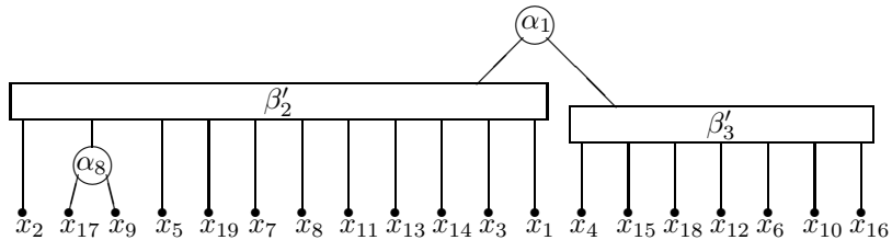
Figure 25: The PQ-tree \mathcal{T} after Step 4
