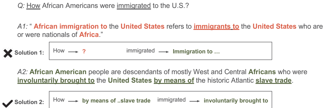
Fig. 1. In the answers A1 and A2 , words in bold represent semantic and syntactic relatedness. Underlined words are: the key words (pattern clues) in Q and corresponding matches in A1 and A2 . Solution 2 fills completely the missing part described in Q .
