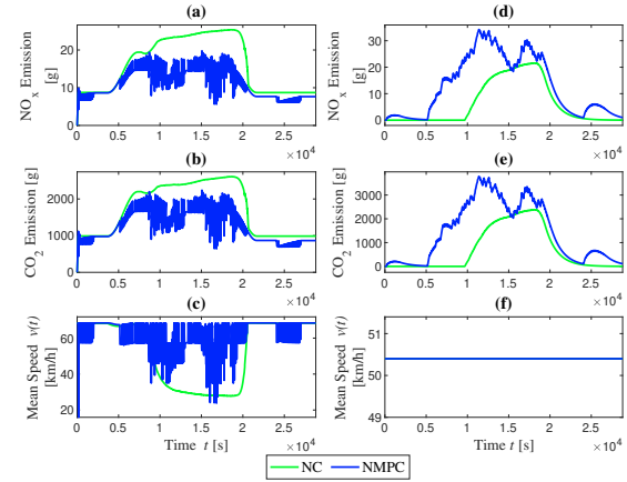
Fig. 5. Response of total emissions and mean speed on the inbound link (left column) and freeway (right column) for nocontrol and NMPC.
