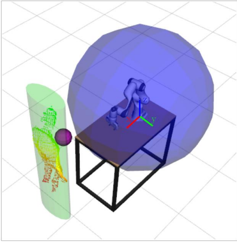
Fig. 4. The human point-cloud and associated circumscribed ellipse and the robot workspace used to calculate separation distance. The purple sphere near the human is the nearest point to the robot.
