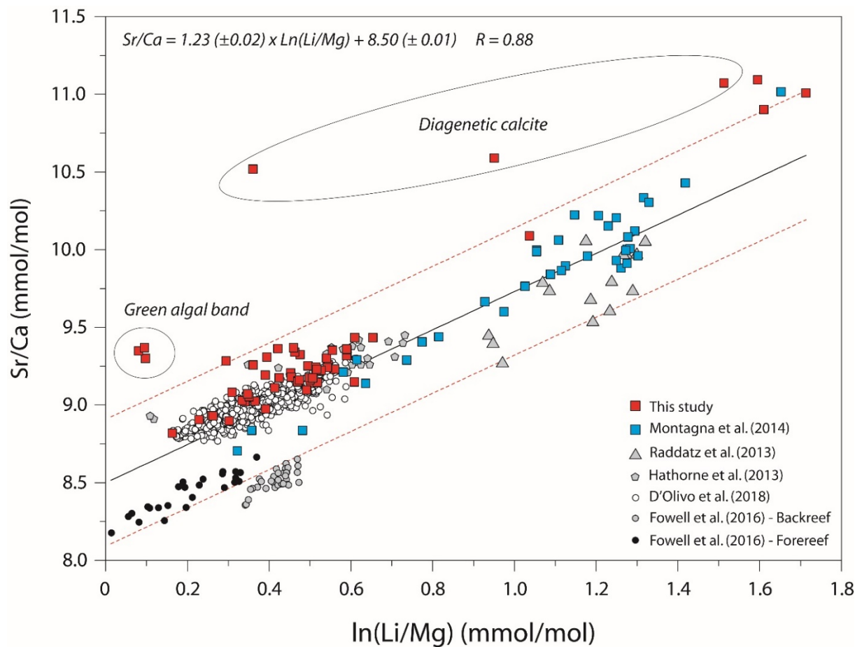
Figure 14. Paired Sr/Ca vs. ln(Li/Mg) values for all the chemically-cleaned samples analysed in the present study (red squares), plotted together with data from Hathorne et al. (2013) (Sr/Ca values are from Felis et al., 2009), Raddatz et al. (2013), Montagna et al. (2014), Fowell et al. (2016) and D'Olivo et al. (2018). Linear regression and 99% prediction intervals were calculated using all the available data, excluding the samples with detectable calcite.
