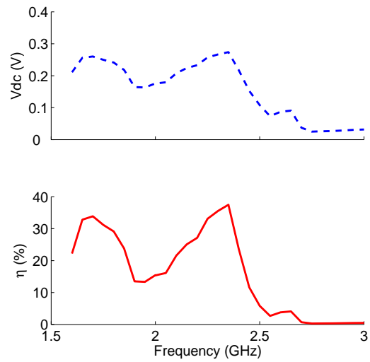
Figure 5. Measured output dc voltage and conversion efficiency against frequency
