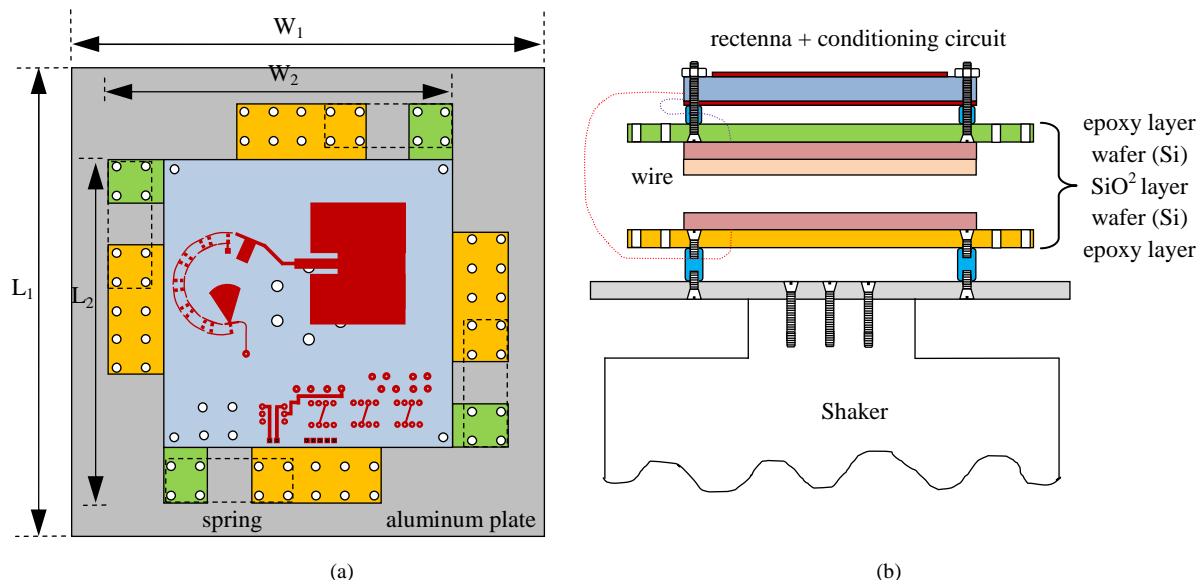
Figure 1. Geometry of the proposed e-VEH: L_1 = W_1 = 150 , L_2 = 120 , W_2 = 120 (dimensions are in mm). Top view (a) and profile view (b).
