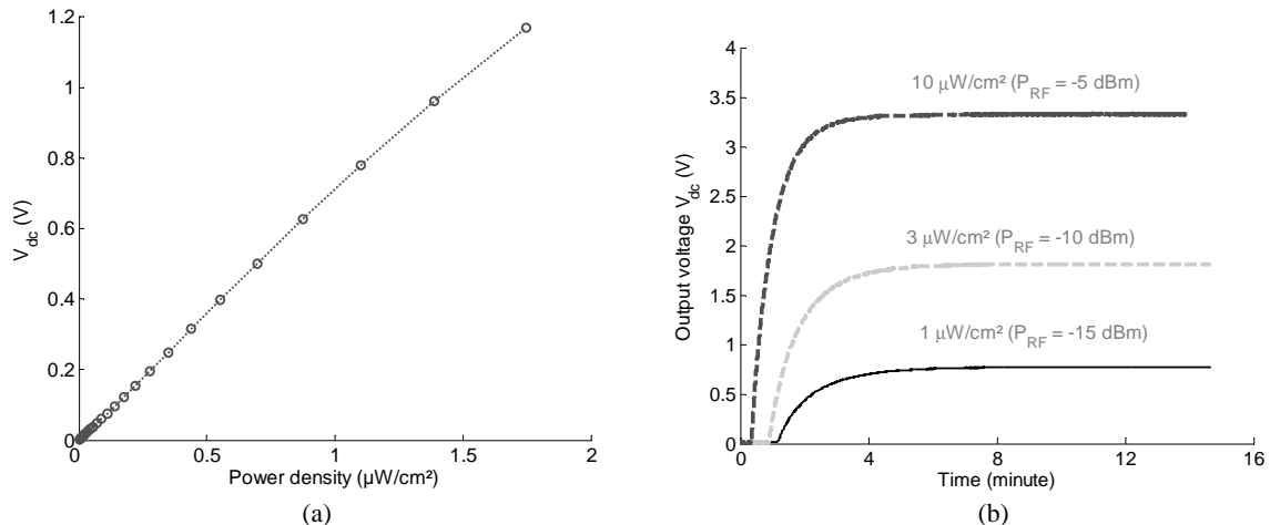
Figure 3. Measured output voltage vs. power density (output load = 100 \text{M}\Omega , f = 2.4 \text{ GHz} ) (a). Measured voltage evolution vs. time over a capacitive load of 1 \text{mF} (b).
