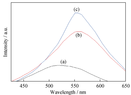
Fig. 6. PL spectra at room temperature of the CuMoO 4 crystals excited at 290 nm after heat treatment at (a) 450, (b) 500, and (c) 550°C.
