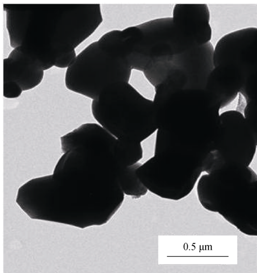
Fig. 5. TEM micrograph of CuMoO 4 powders heat-treated at 450°C for 6 h.
