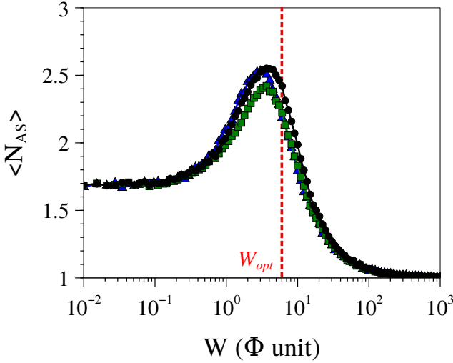
FIG. 4: Mean number \langle N_{AS} \rangle of the active states versus the disorder strength W for \Gamma = 1\Phi (black circles), \Gamma = \Gamma_{opt} = 6\Phi (green squares) and \Gamma = 15\Phi (blue triangles). Each point of the graph is the result of a statistic realized over N_C = 2000 configurations.
